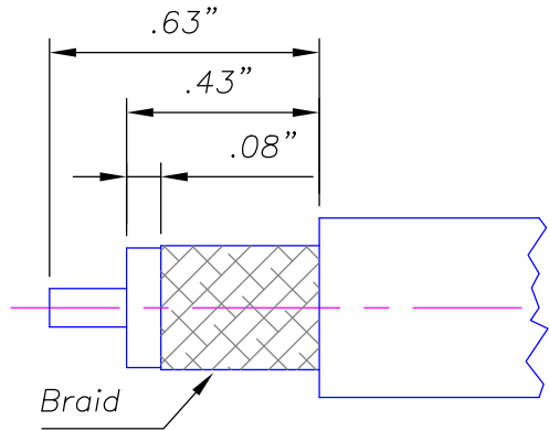
CABLE TRIMMING DETAILS For RG8, 213 & similar cables
